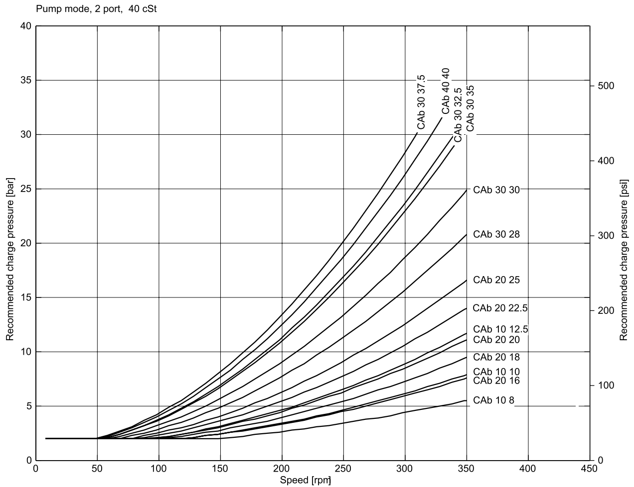
Fig. 6: Recommended charge pressure for motor working in braking mode, Hägglunds CAb 2-port connection. Valid for oil viscosity 40 cSt.
