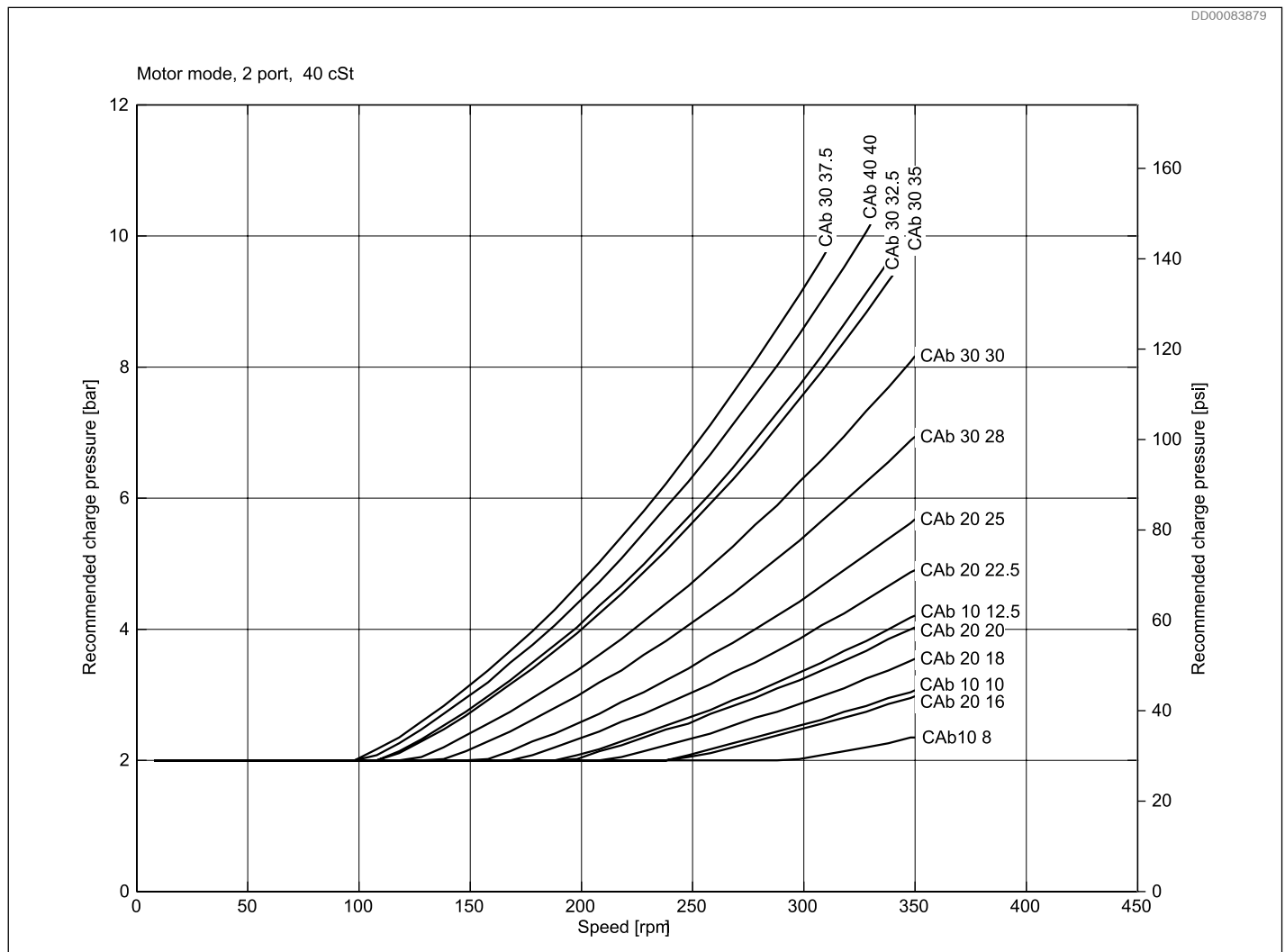
Fig. 5: Recommended charge pressure for motor working in driving mode, Hägglands CAb 2-port connection. Valid for oil viscosity 40 cSt.
