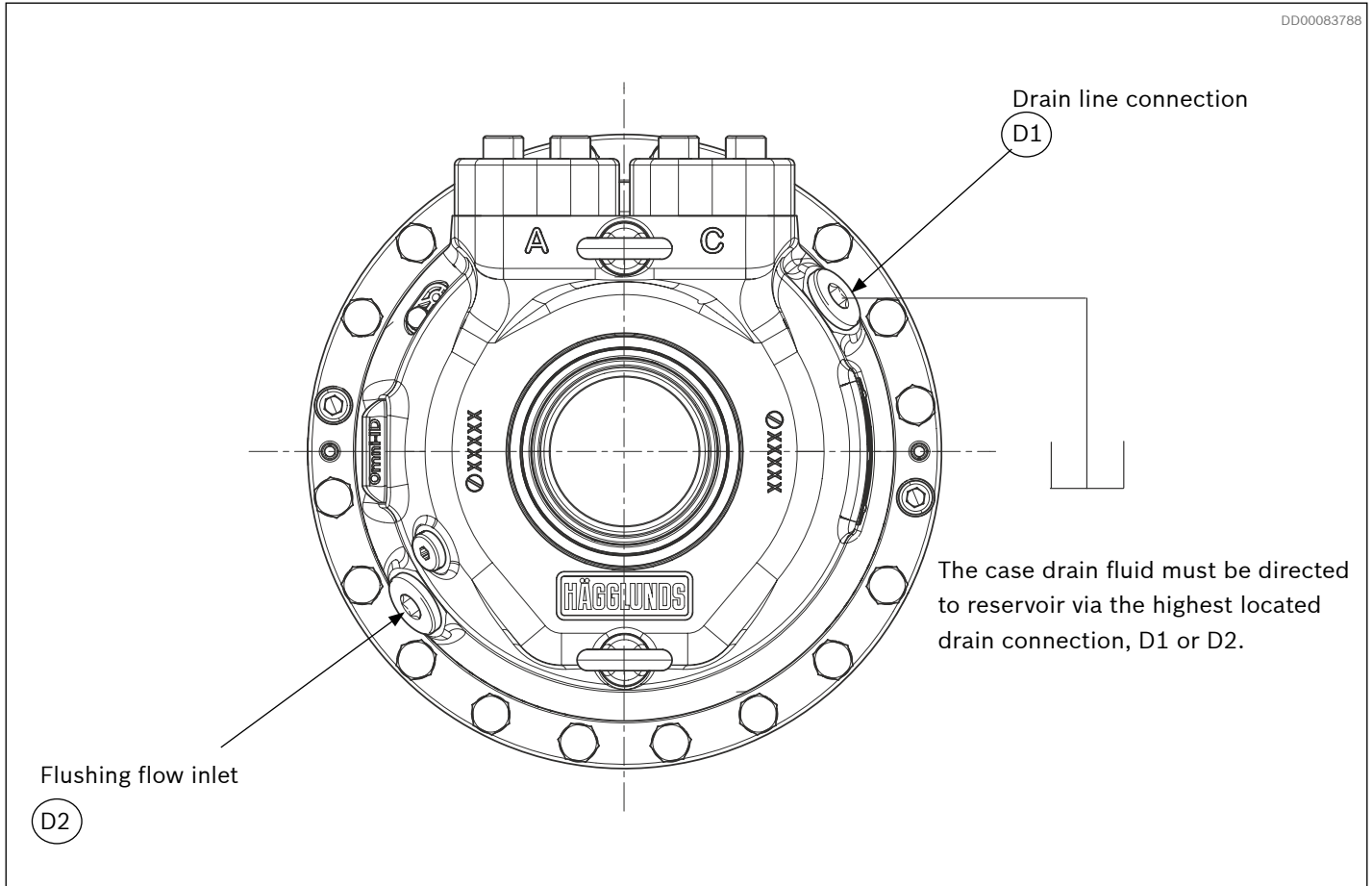
Fig. 24: Horizontal mounting
