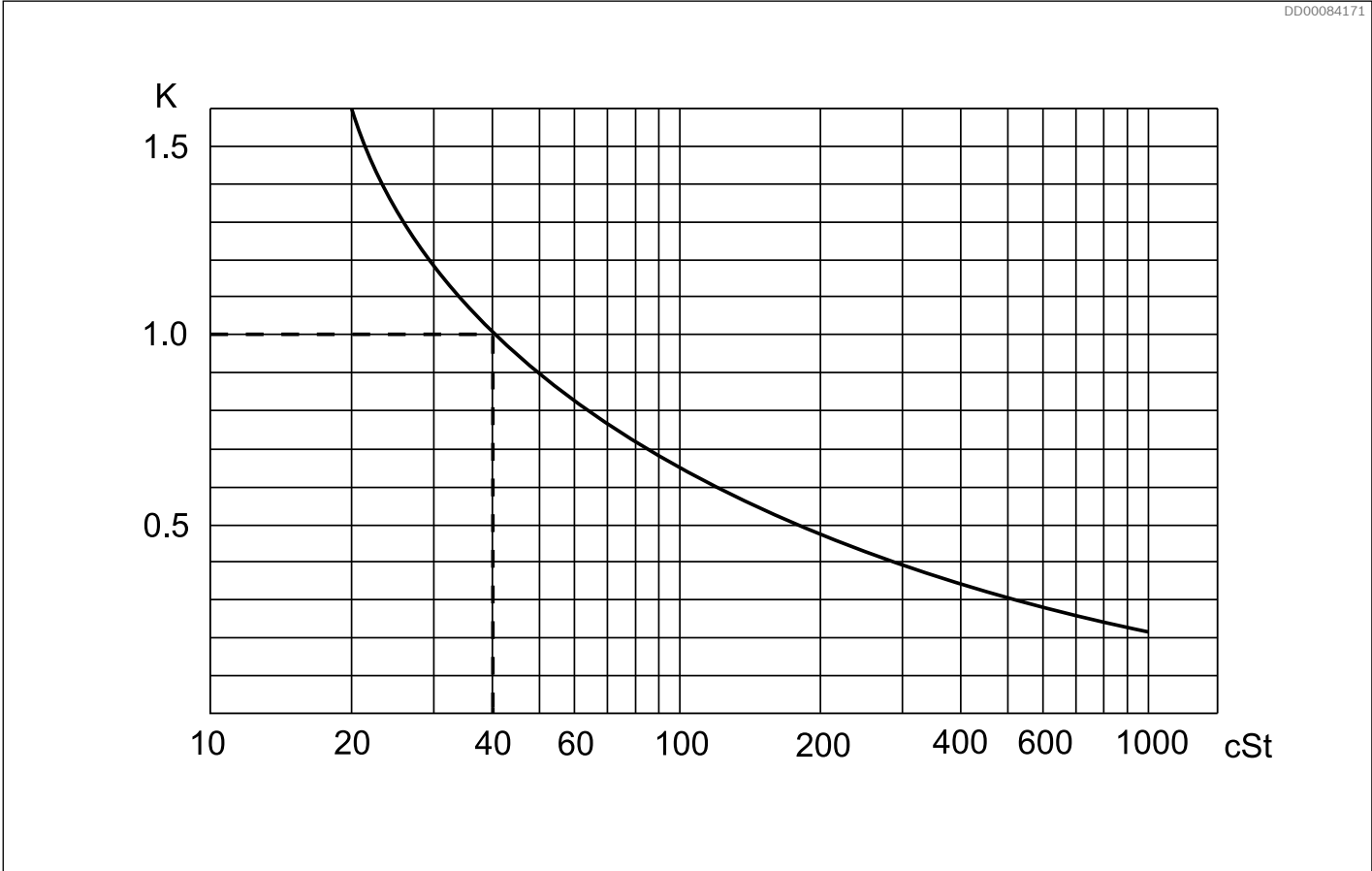
Fig. 29: Viscosity factor K
